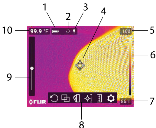
Figure 4.5 Videoscope display.
