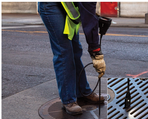
Figure 6.2 Insert the probe into the test area.
